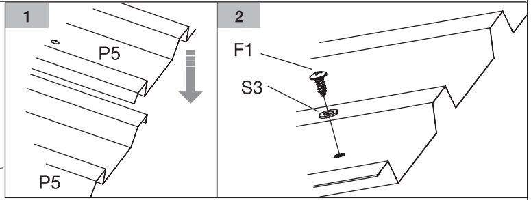
S3 x 12
